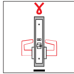
Electrically locking/unlocking both levers, no cylinder
