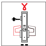
Electrically locking/unlocking outside lever, outside cylinder
