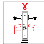
Electrically locking/unlocking both levers, double cylinder
